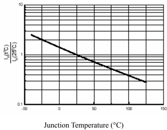
FIGURE 7-Typical Holding Current
